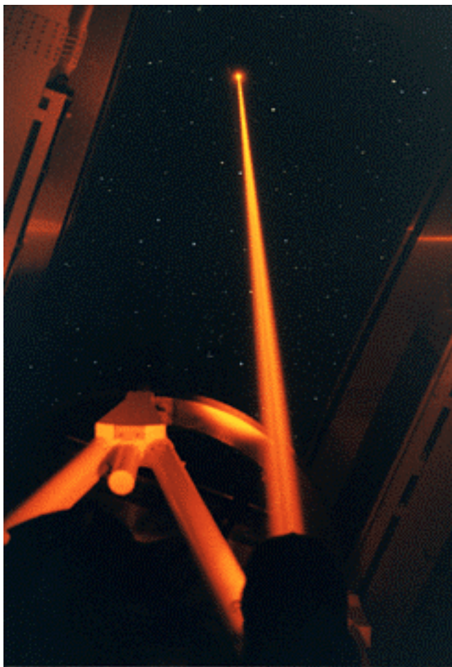
Figure 2. The ALFA laser beam projection.
