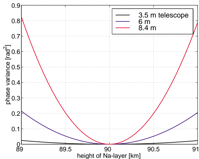
Figure 5. Focus error with laser guide stars for different telescope sizes.
