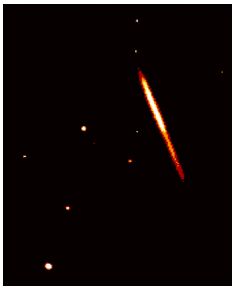
Figure 4. The LGS seen from the side (laser-cigar). The LGS launch telescope and the observing telescope (1.2 m, 60 s exposure time) are 265 m apart. The length of the laser-cigar is about 100'' on the sky which corresponds to about 12 km under the assumptions that the laser-cigar starts at an altitude of 75 km and the launch telescope points perfectly to zenith.
