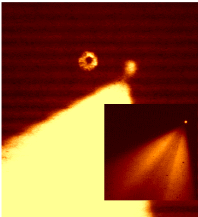
Figure 3. Rayleigh cone, LGS, and defocused NGS. The small image in the lower right shows a better focused LGS than the large image. The pupil-like defocused star SAO 055924 has a V-magnitude of 9.5.
