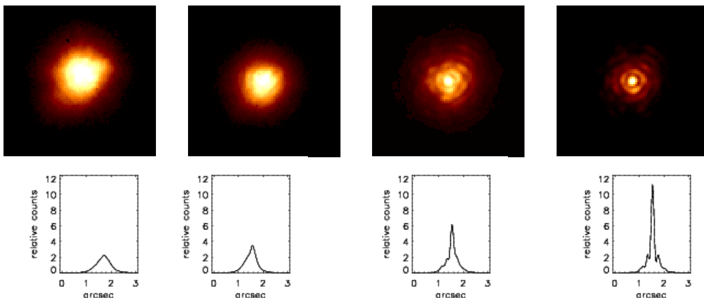
Figure 6 a-d (from left to right). a) Open loop 50 sec K-band image of SAO 68075. FWHM: 0.65". b) 50 sec image with tip-tilt corrected on the star. FWHM: 0.49". c) 200 sec (40 co-added images) exposure, with tip-tilt corrected on the star and high order correction on the laser guide star. FWHM: 0.19" and 12.8% Strehl. d) During the very best 10 sec, a Strehl number of 23% and a full diffraction limited PSF was obtained (FWHM: 0.14"). The first diffraction ring is clearly visible.
